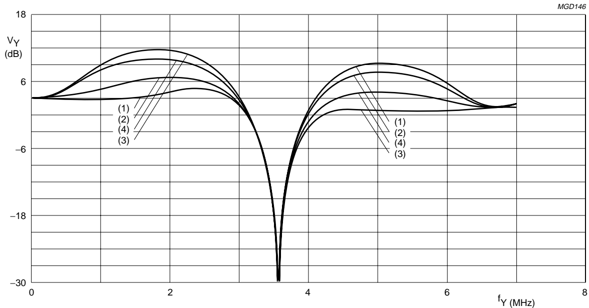
Fig.51 Luminance control SA 09H, 3.58 MHz Trap/CVBS mode, prefilter off, different aperture band-pass centre frequencies.
