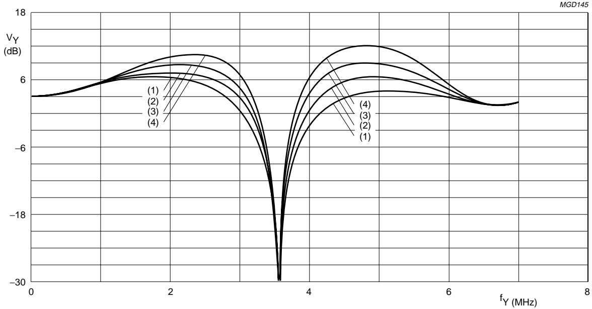
Fig.50 Luminance control SA 09H, 3.58 MHz Trap/CVBS mode, prefilter on, different aperture factors.
